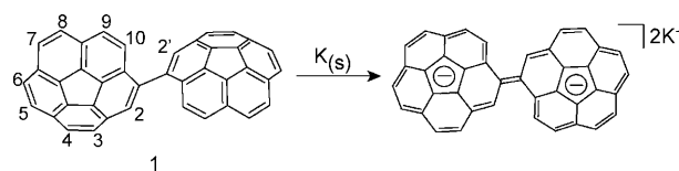
Scheme 1. Reduction of bicorannulenyl ( 1 ) with elemental potassium.
