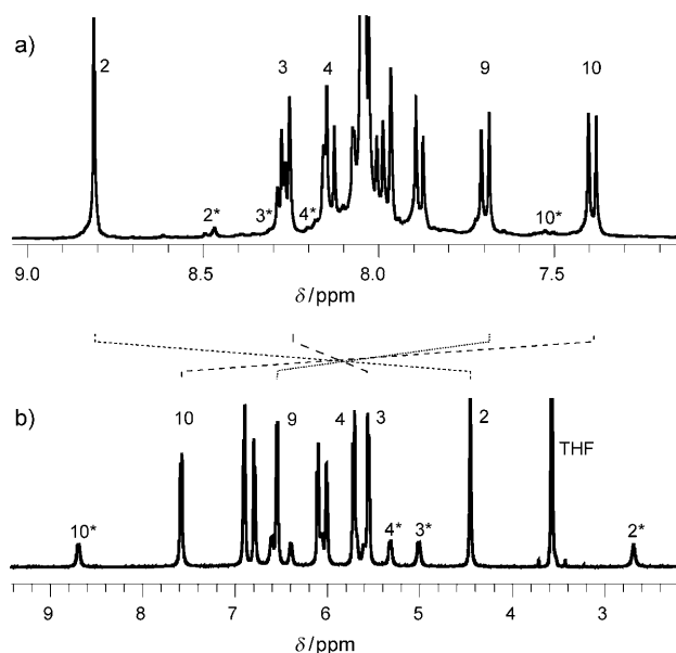
Figure 1. ^1\text{H} NMR spectra of a) 1 and b) 1 2- at 190 K. Representative signals are annotated (see Scheme 1 for numbers, minor isomer signals are marked with *). Note the change in the spectral range.
